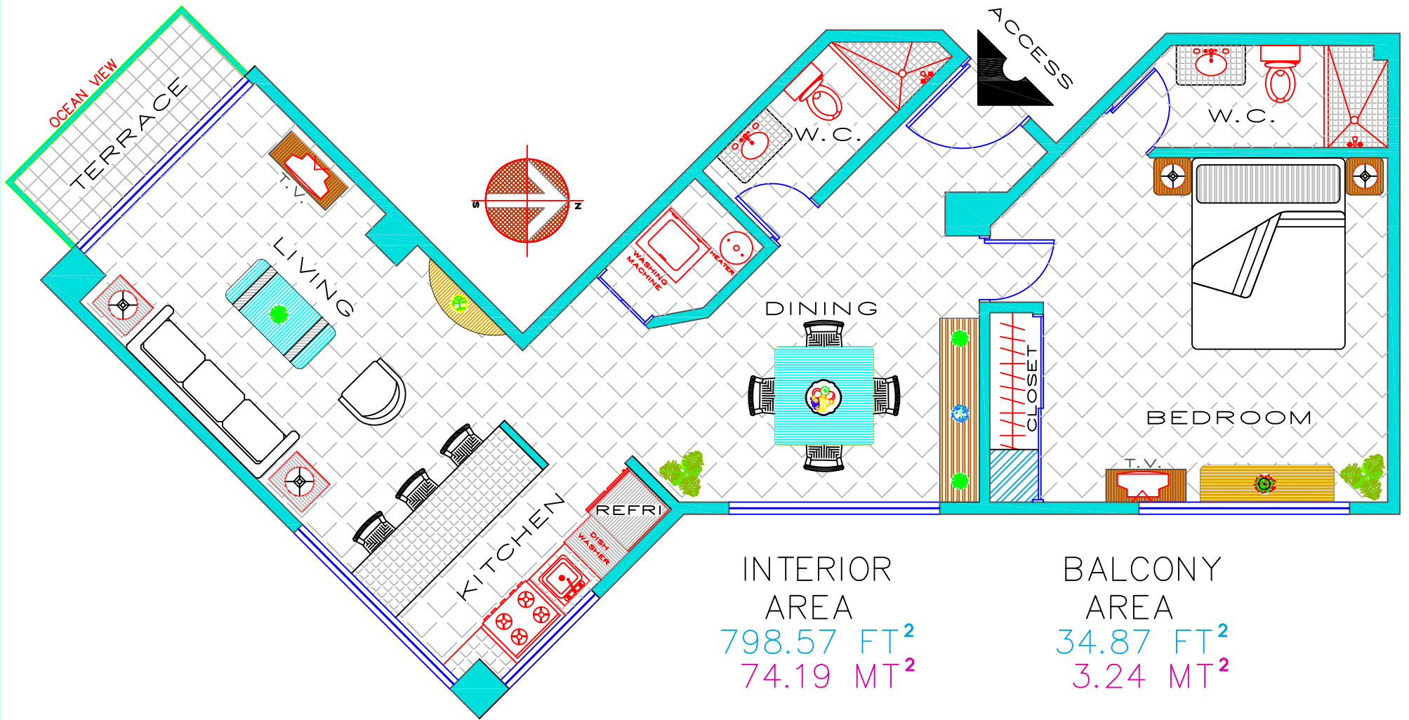
ARCHITECTURAL PLAN T-1 1003 FURNITURE'S
