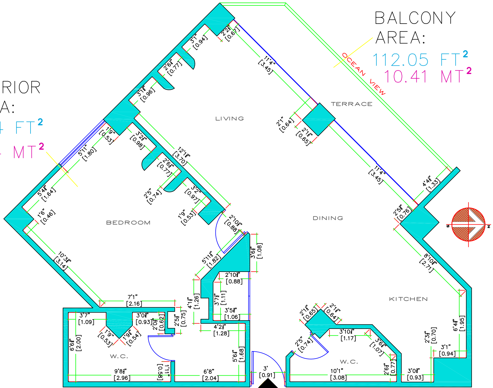
ARCHITECTURAL PLAN CM-309 MEASURE'S
