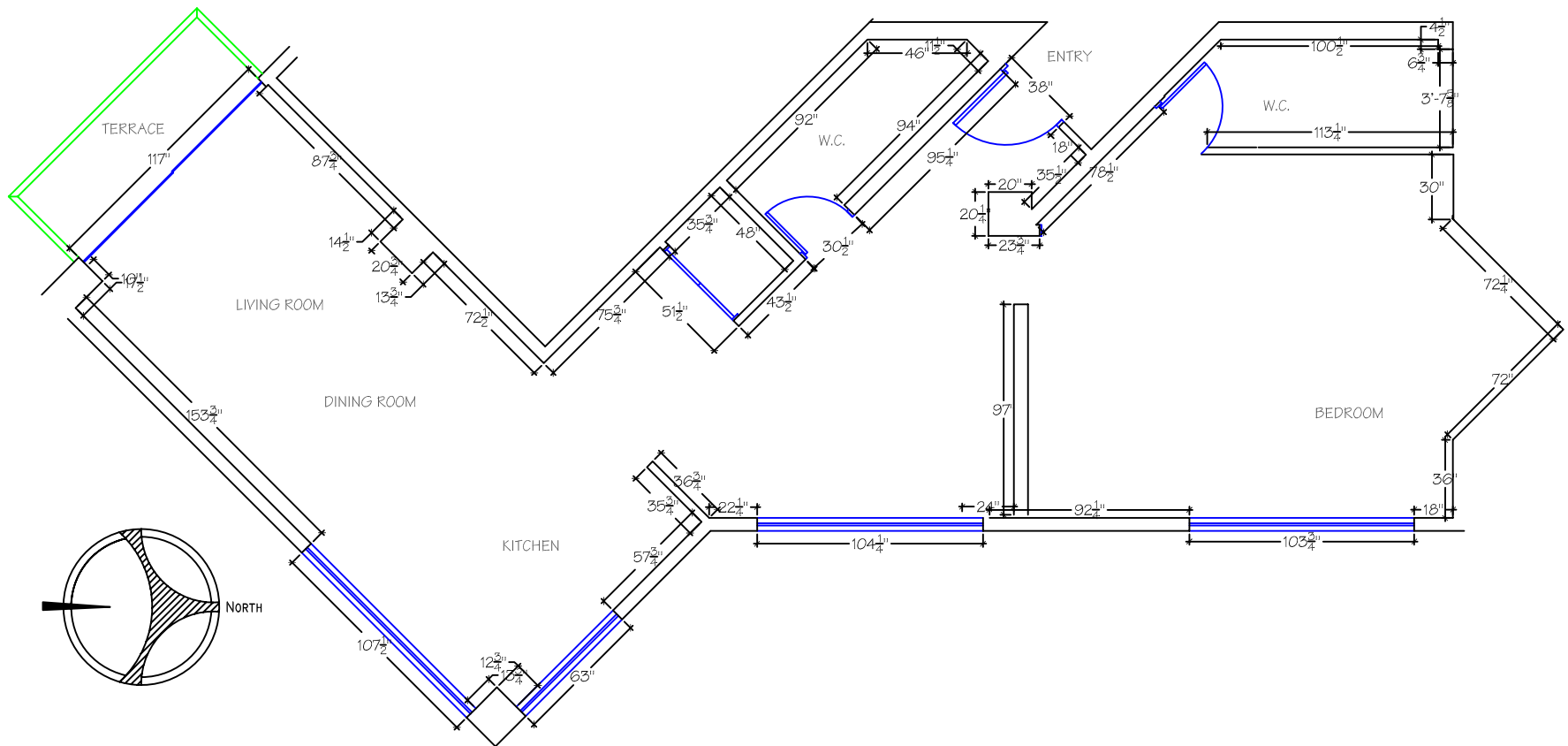
ARCHITECTONIC PLAN T-II 403 MEASURES
