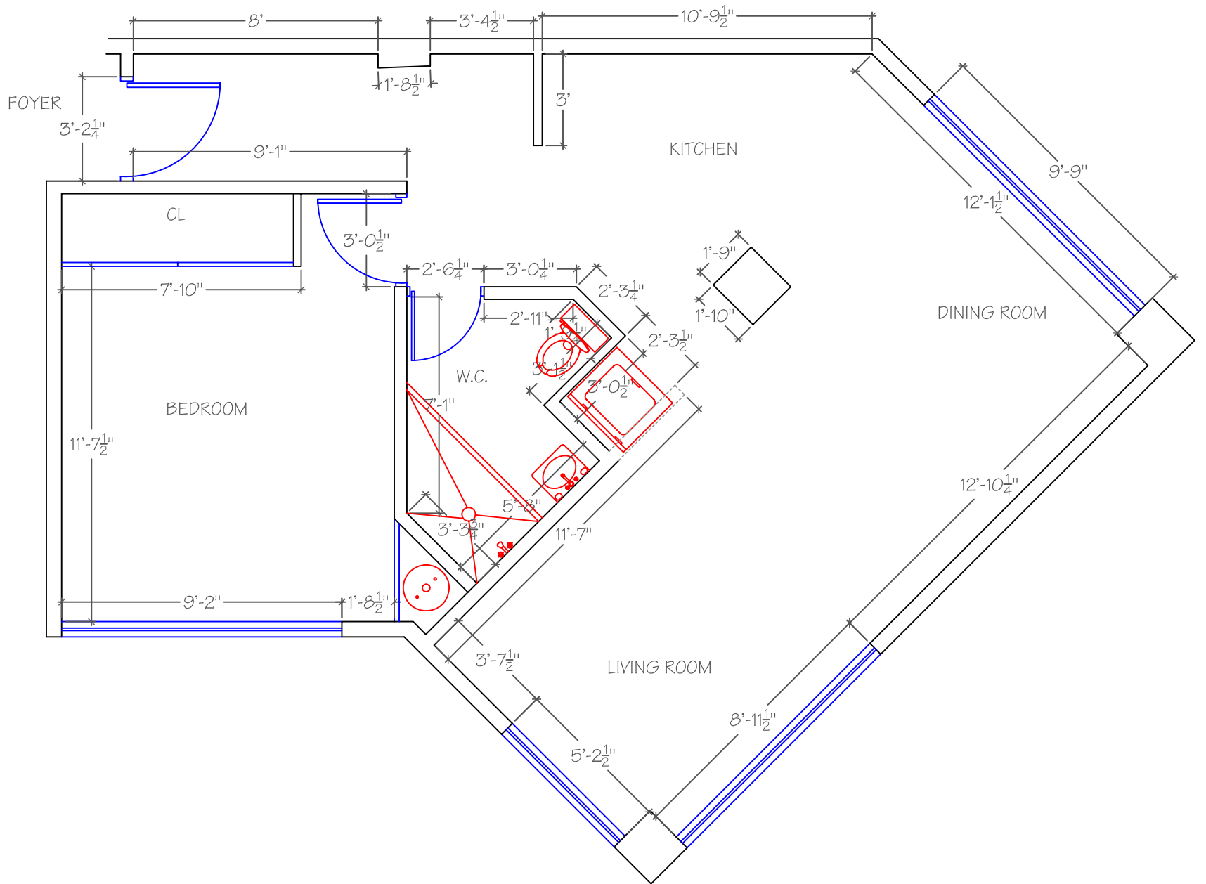
ARCHITECTONIC PLAN T-II 104 MEASURES & FURNITURE
