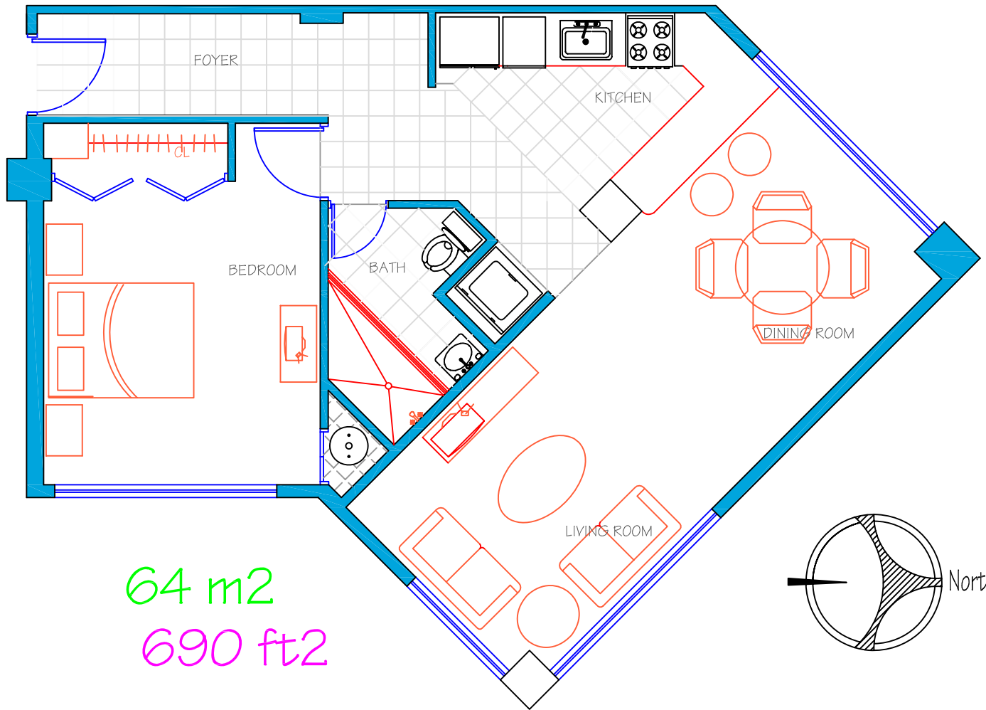
ARCHITECTONIC PLAN T-II 104 FURNITURE
