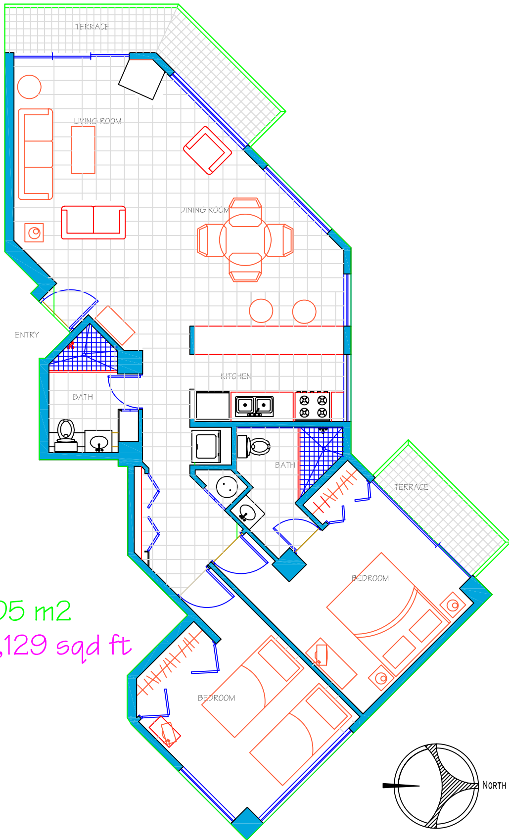
ARCHITECTONIC PLAN T-1 702 FURNITURE
