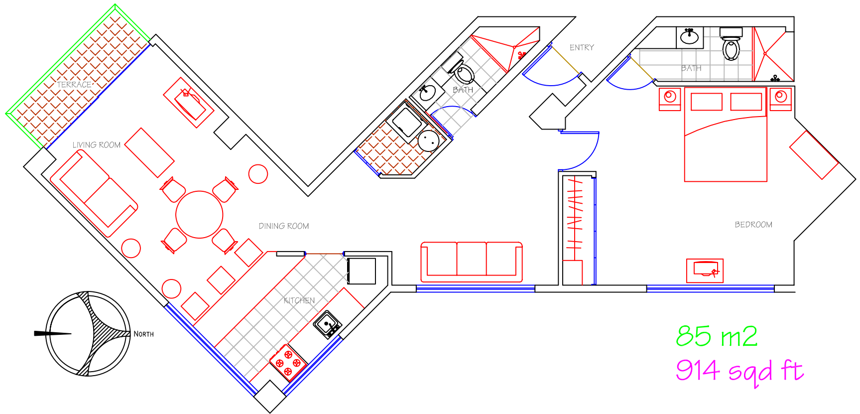
ARCHITECTONIC PLAN T-1 203 FURNITURE
