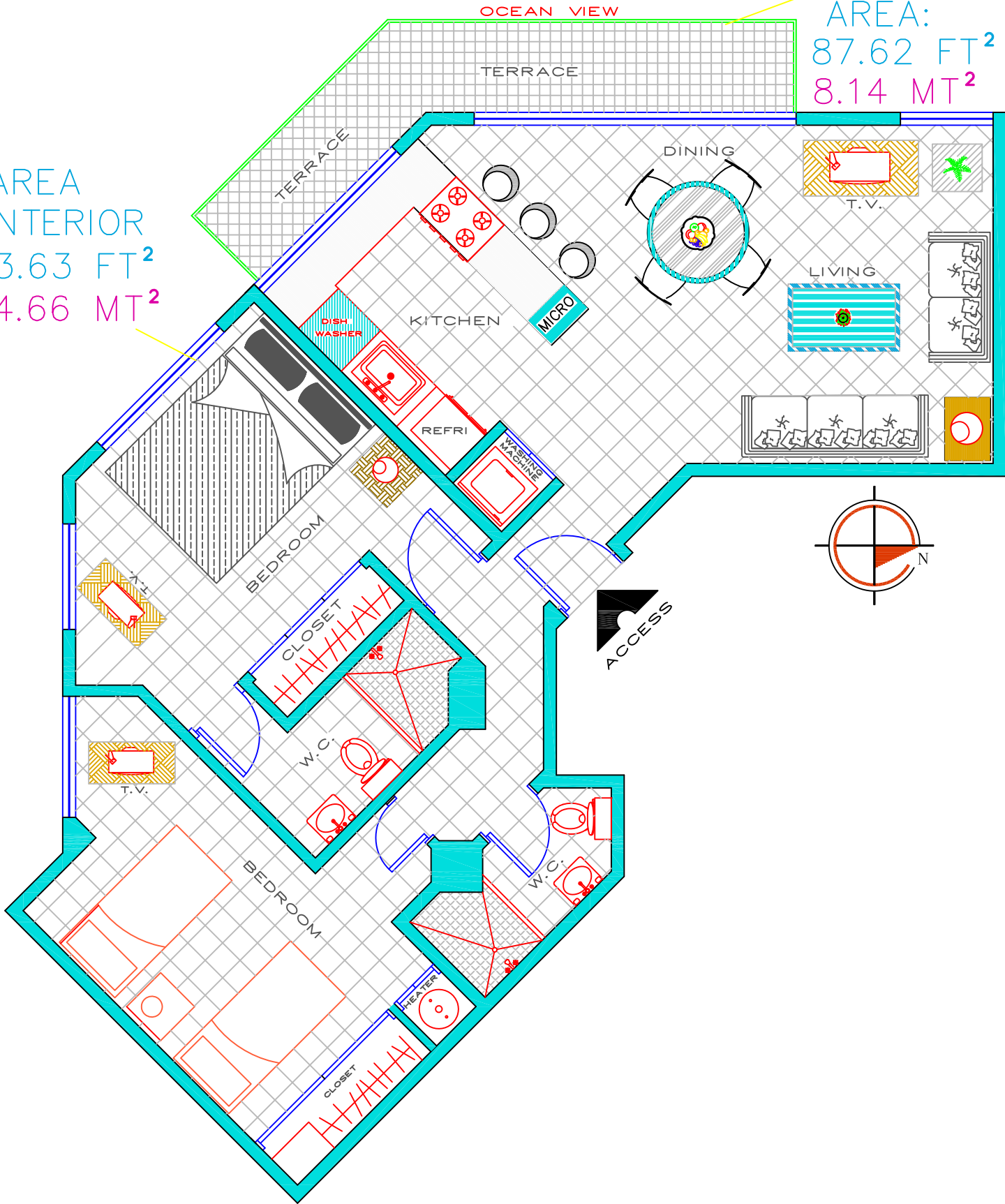
ARCHITECTURAL PLAN T-I 1001 FURNITURES
