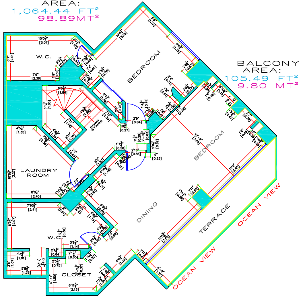
SECOND FLOOR
