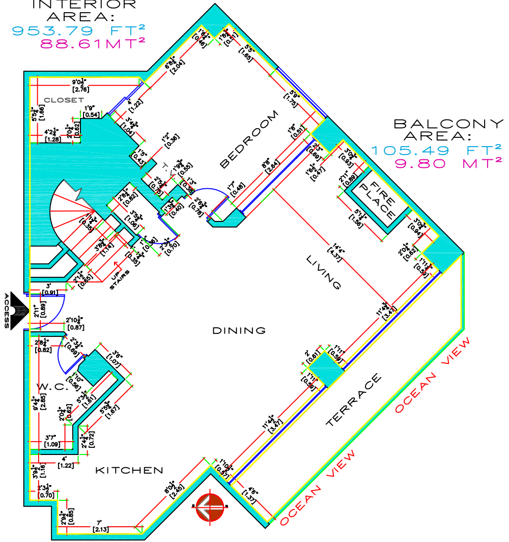
FIRST FLOOR
