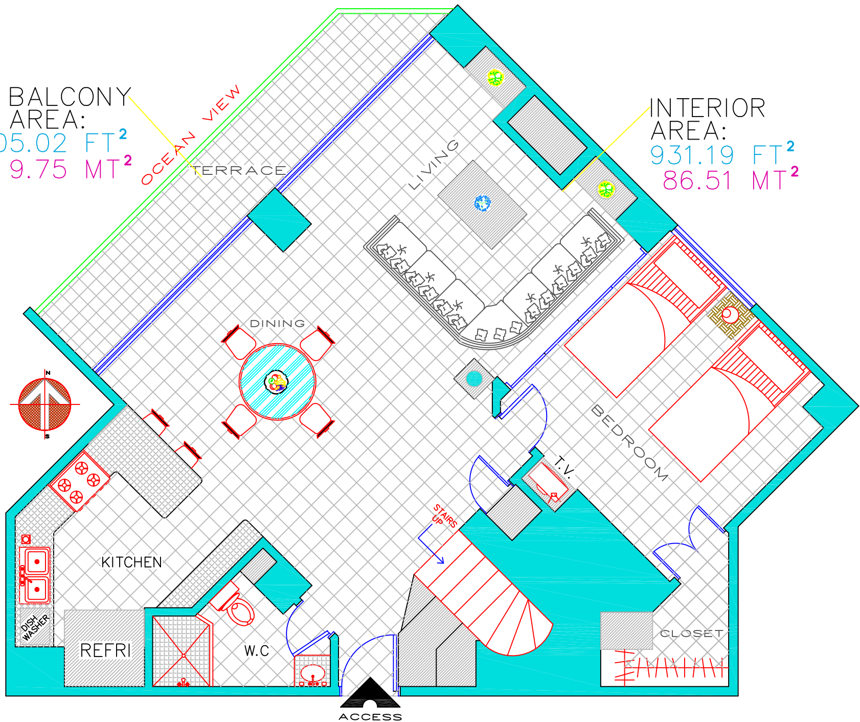
ARCHITECTURAL PLAN CM-912 FIRST FLOOR FURNITURES
