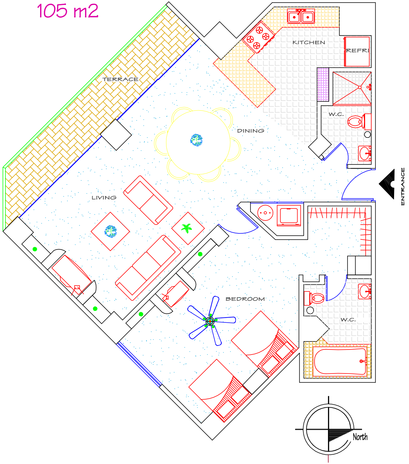
ARCHITECTURAL PLAN CM-911 FURNITURES
