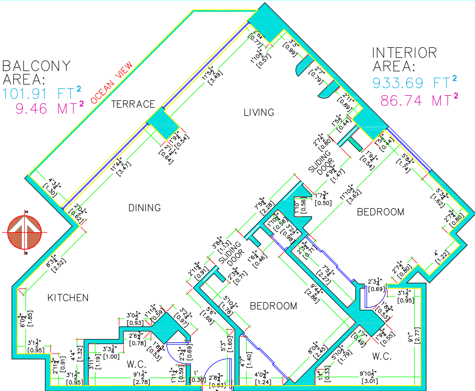
ACCESS ARCHITECTURAL PLAN CM-910 MEASUREMENTS
