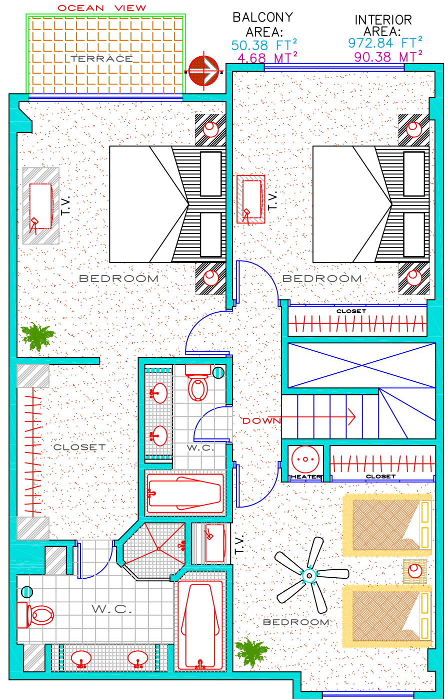
ARCHITECTURAL PLAN CM-902 FURNITURE'S SECOND FLOOR
