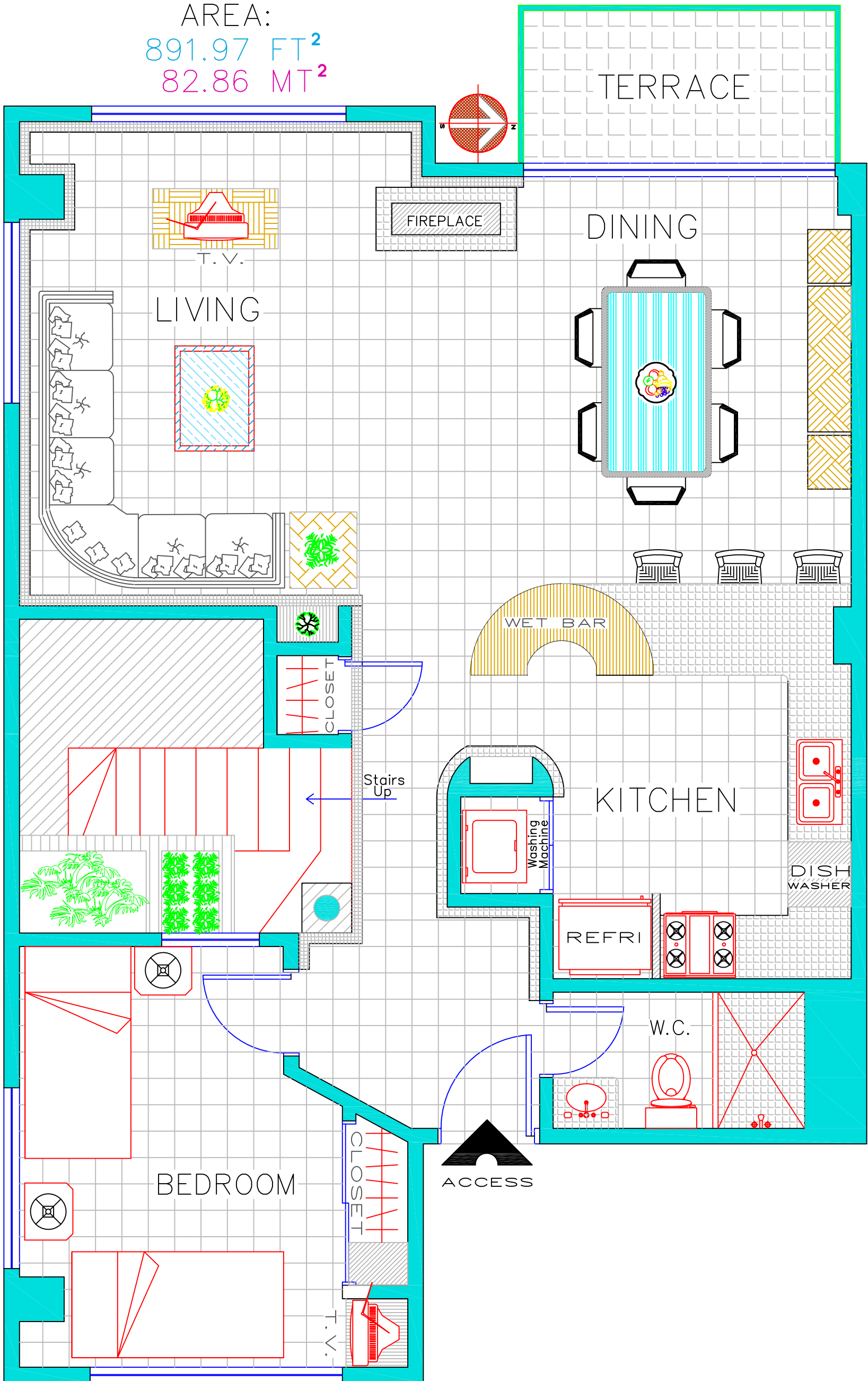
ARCHITECTURAL PLAN CM-901 FURNITURE'S FIRST FLOOR
