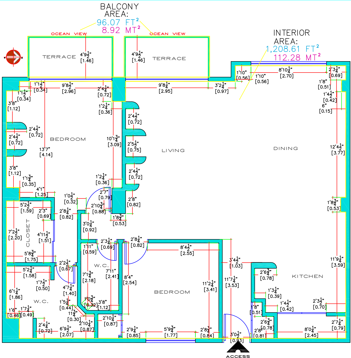
ARCHITECTURAL PLAN CM-803 MEASURE'S
