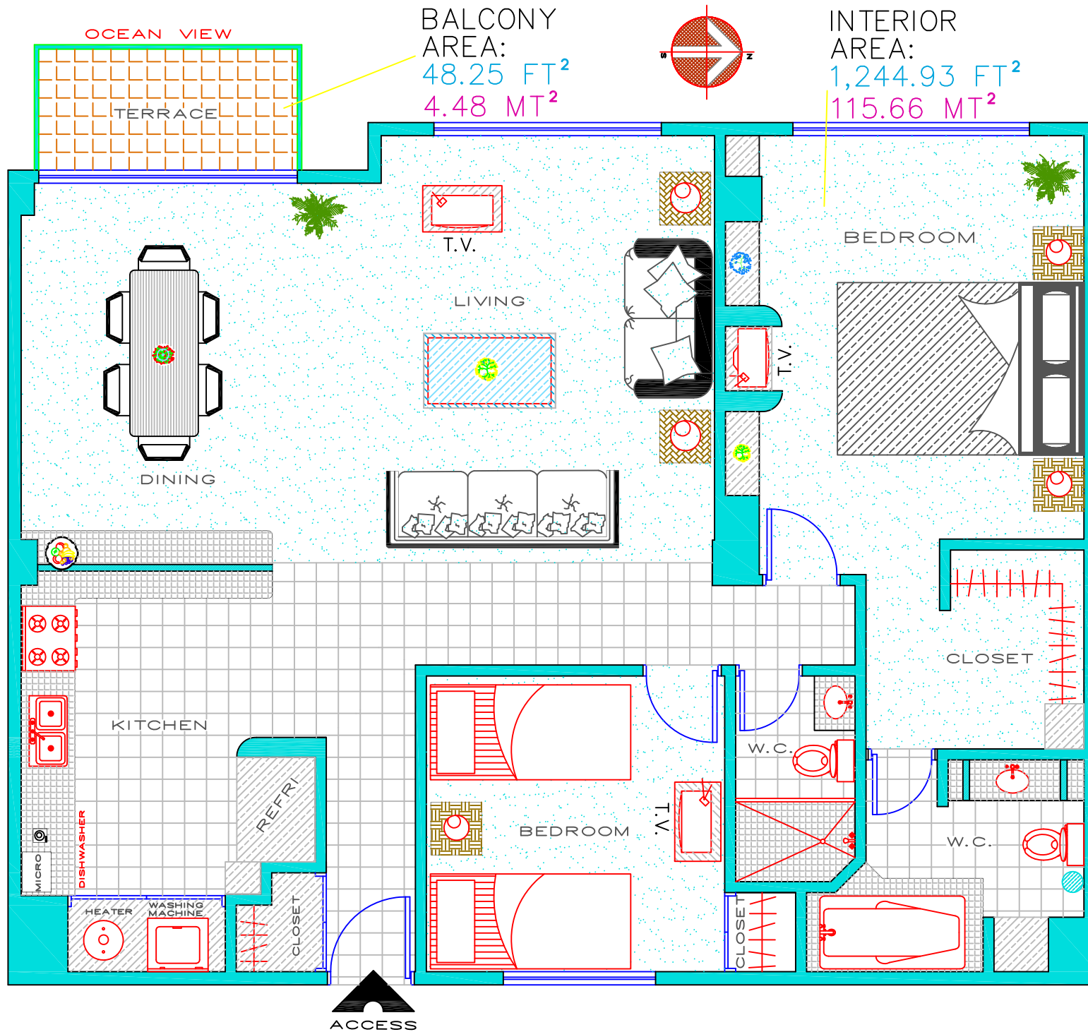
ARCHITECTURAL PLAN CM-802 FURNITURE'S
