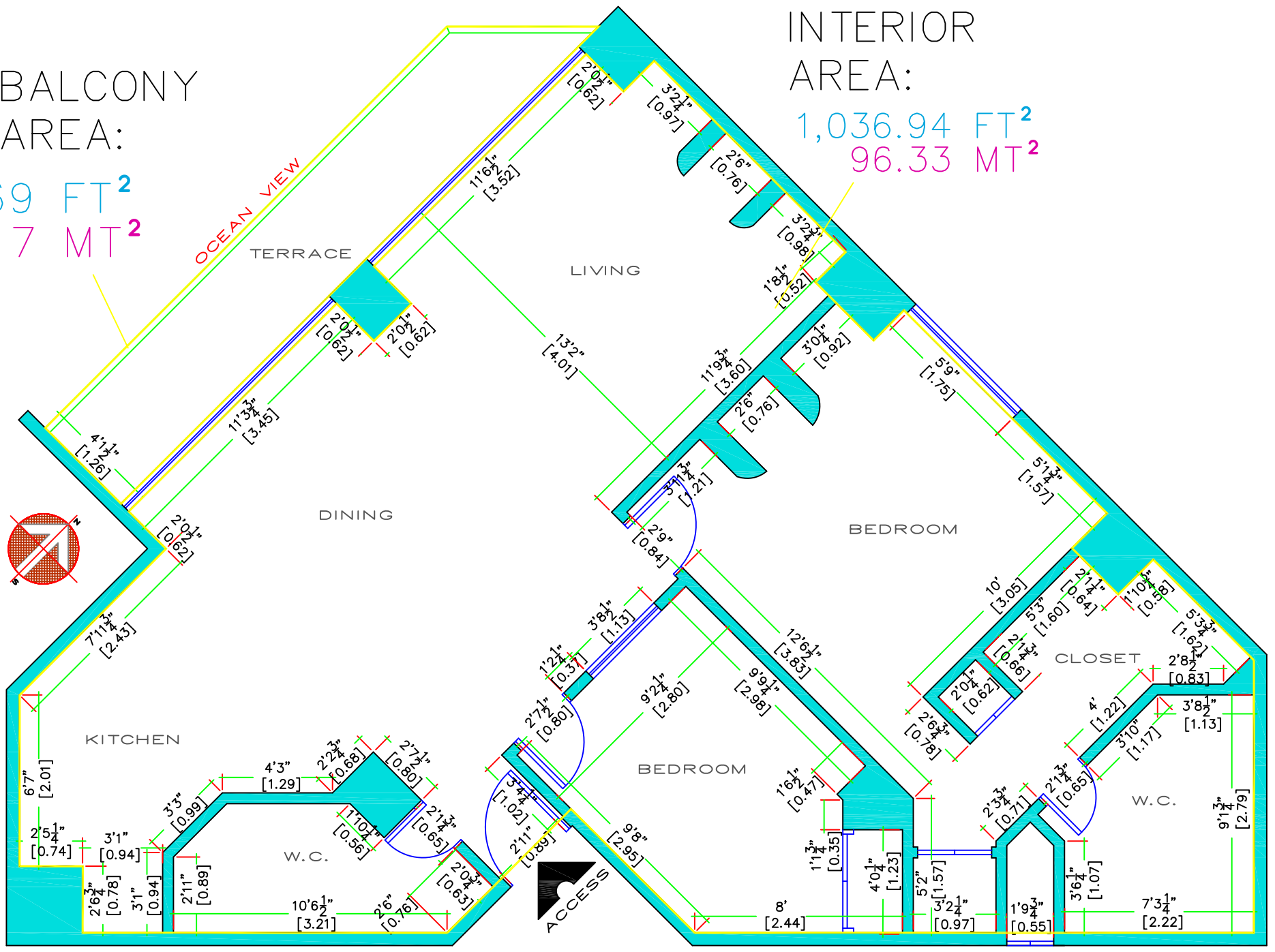
ARCHITECTURAL PLAN CM-608 MEASURE'S
