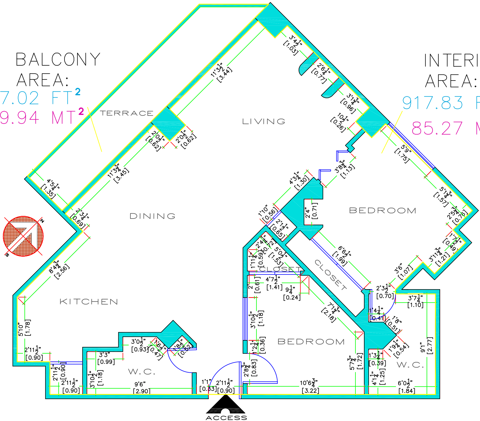
ARCHITECTURAL PLAN CM-510 MEASURES
