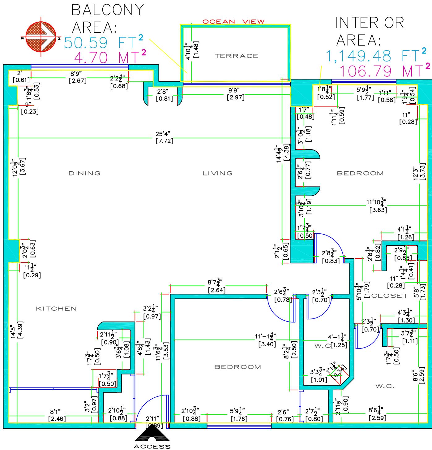
ARCHITECTURAL PLAN CM-504 MEASURE'S
