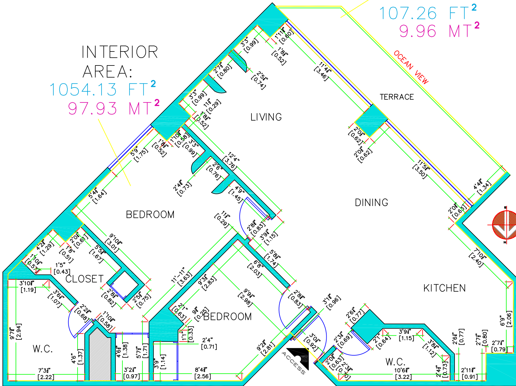
ARCHITECTURAL PLAN CM-407 MEASURES
