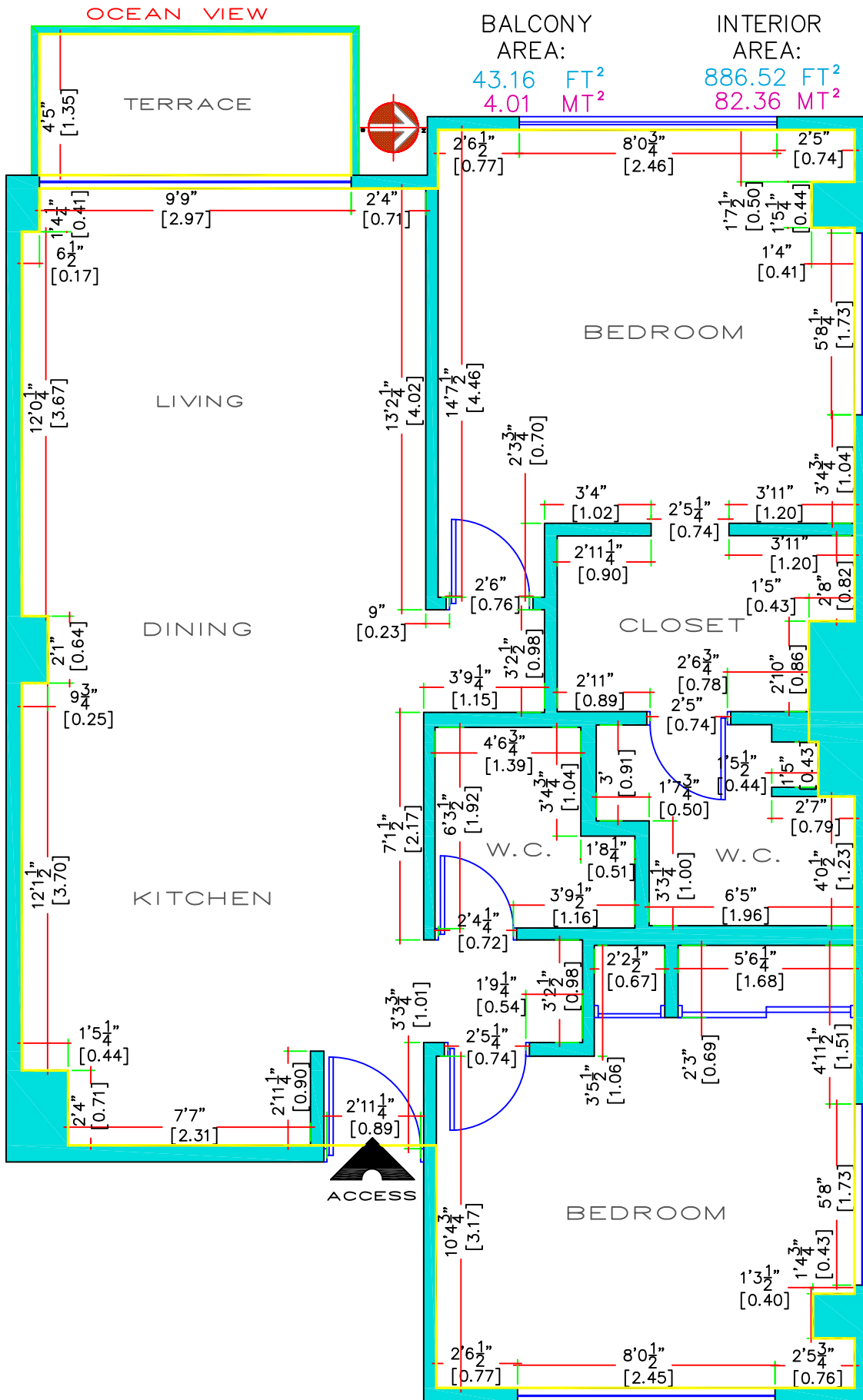
ARCHITECTURAL PLAN CM-406 MEASURE'S
