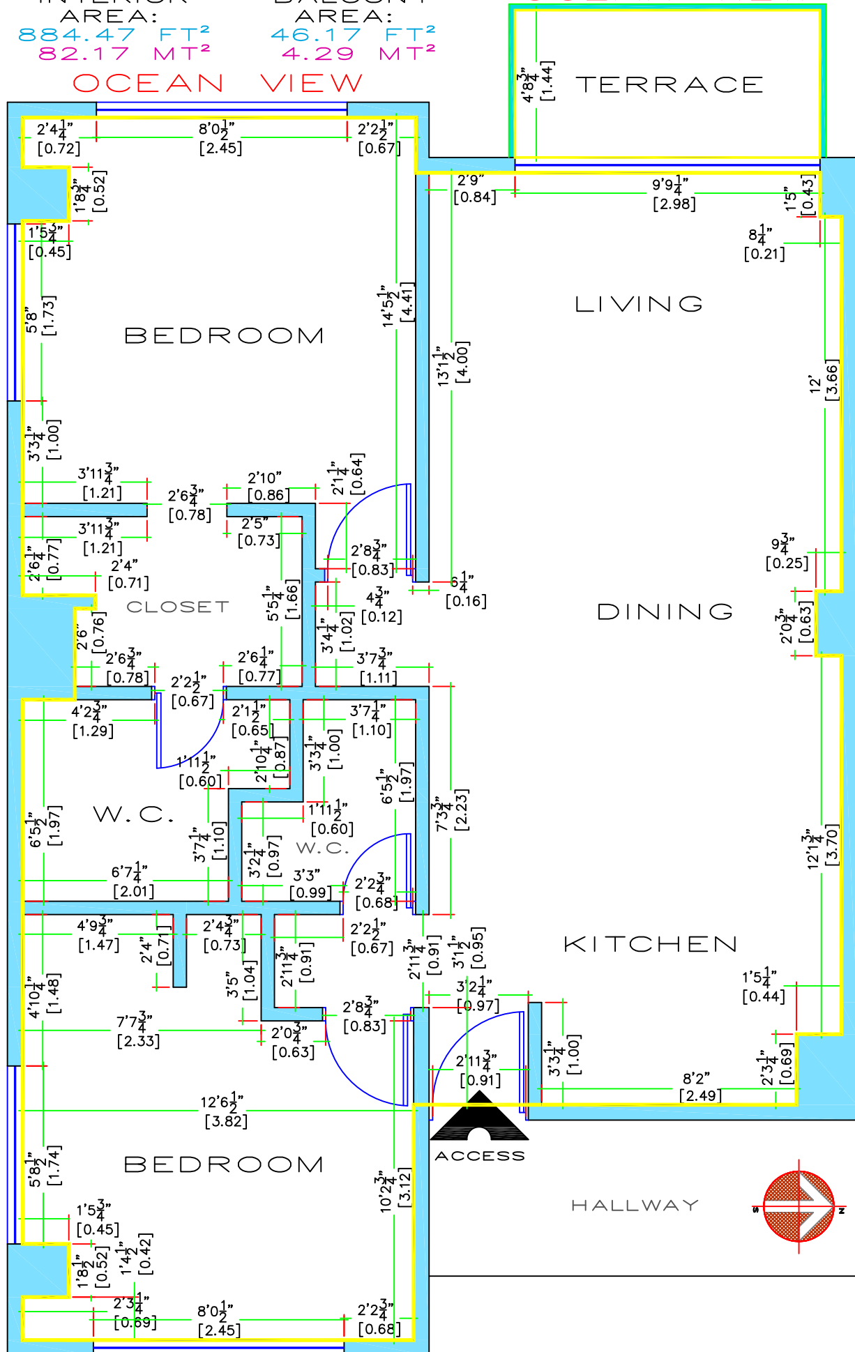
ARCHITECTURAL PLAN CM-401 MEASURE'S
