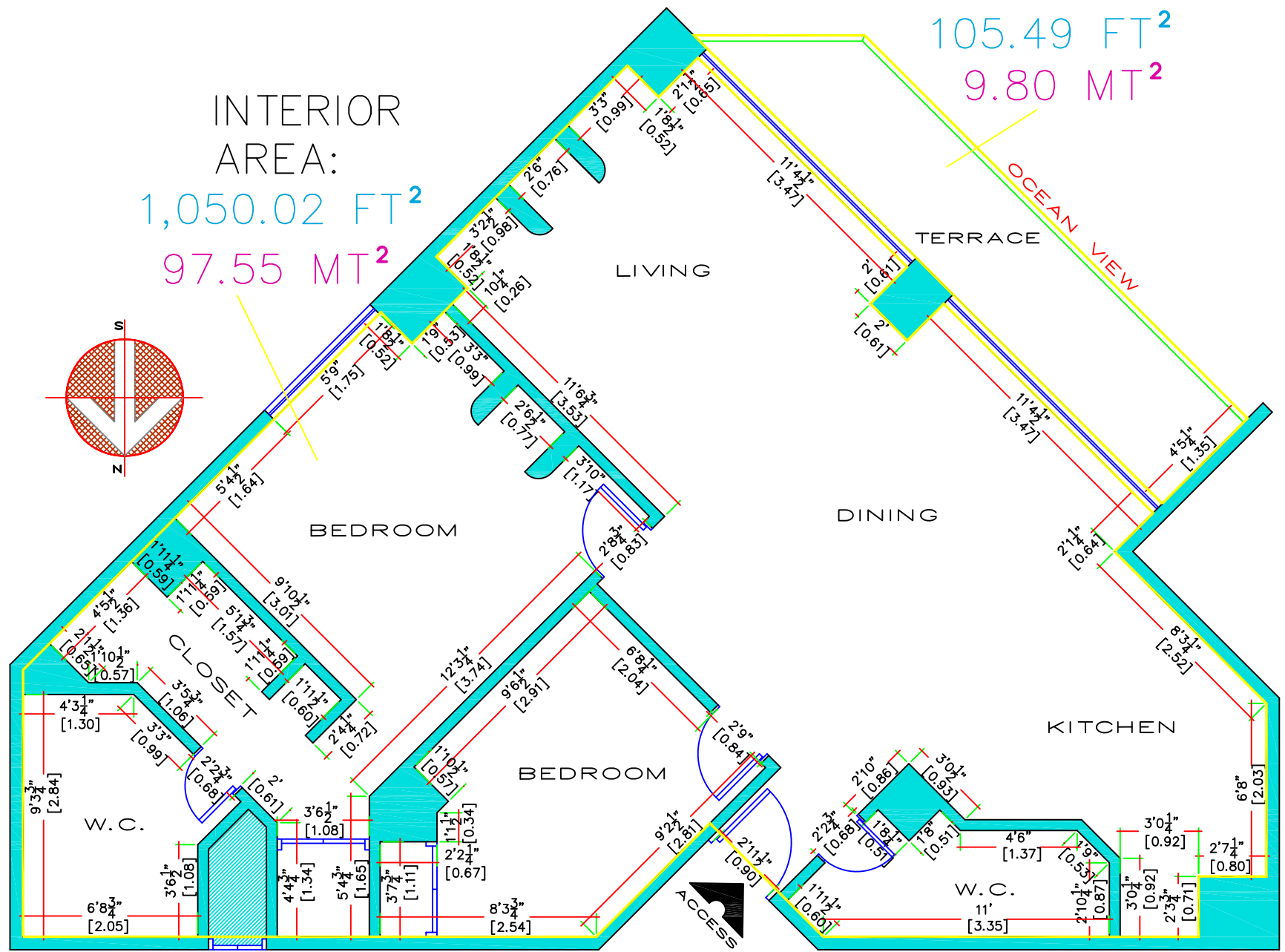
ARCHITECTURAL PLAN CM-307 MEASURE'S
