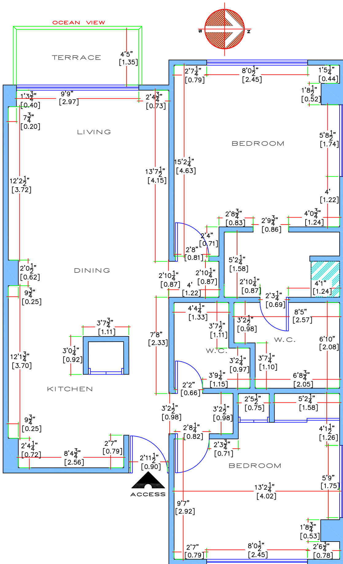
ARCHITECTURAL PLAN CM-306 MEASURE'S
