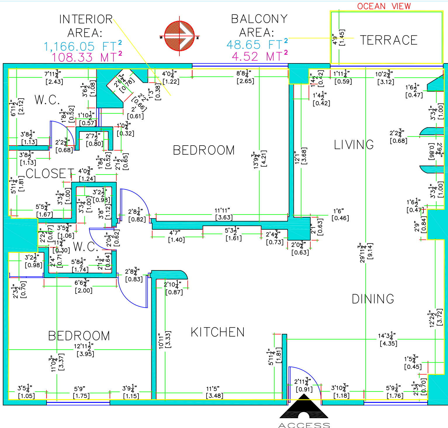
ARCHITECTURAL PLAN CM-305 MEASURES
