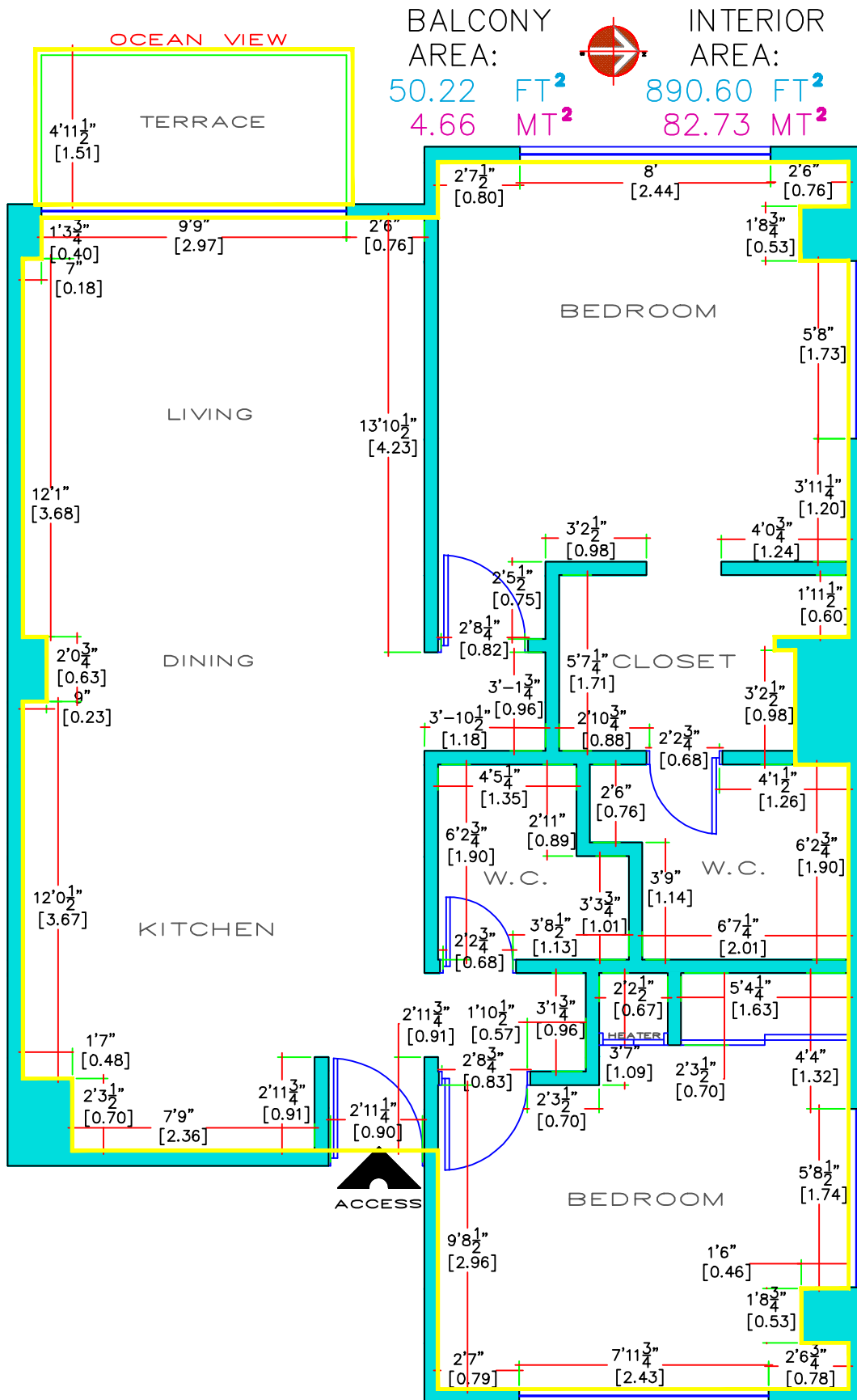
ARCHITECTURAL PLAN CM-206 MEASURES
