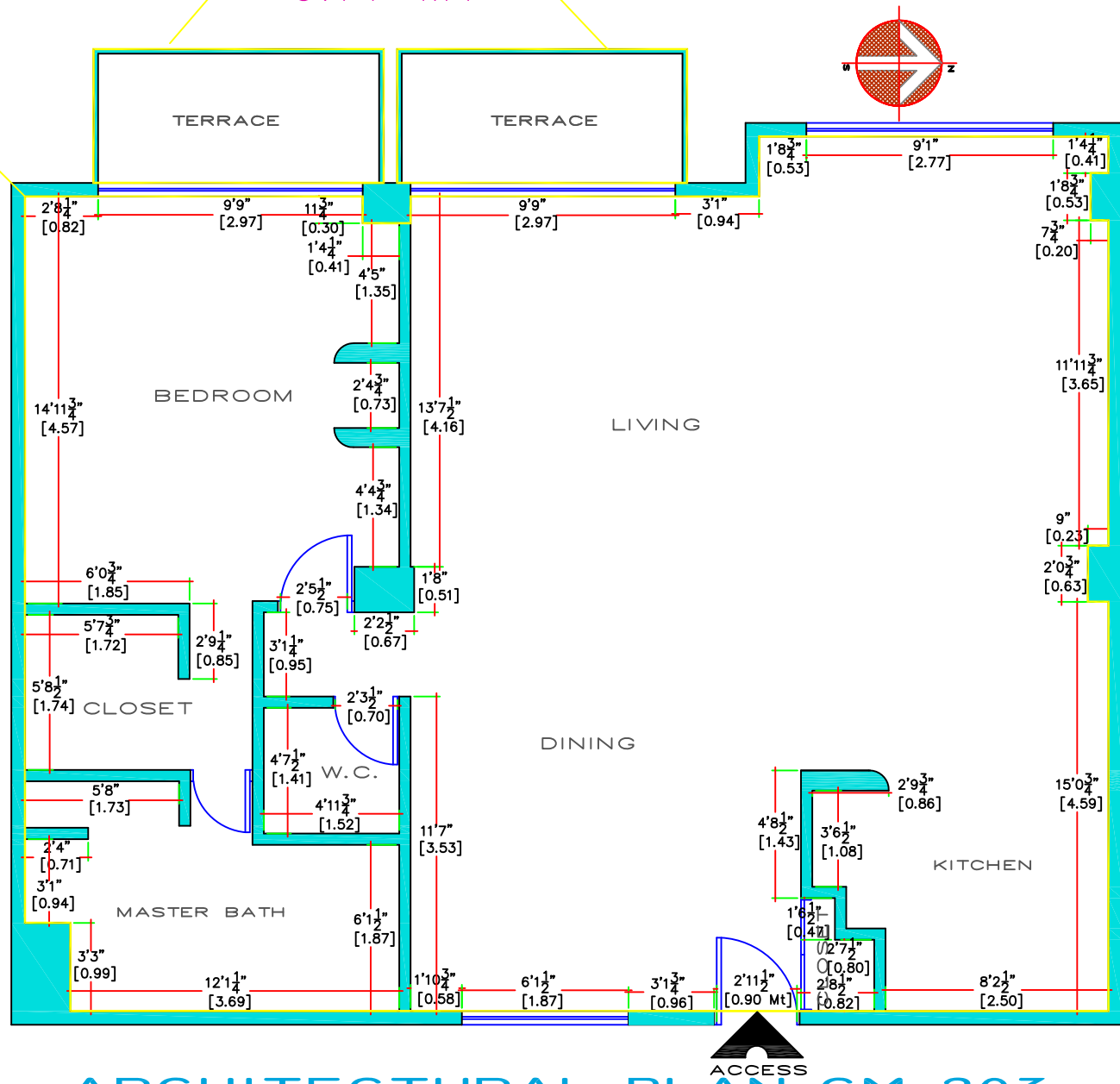
ARCHITECTURAL PLAN CM-203 MEASURE'S
