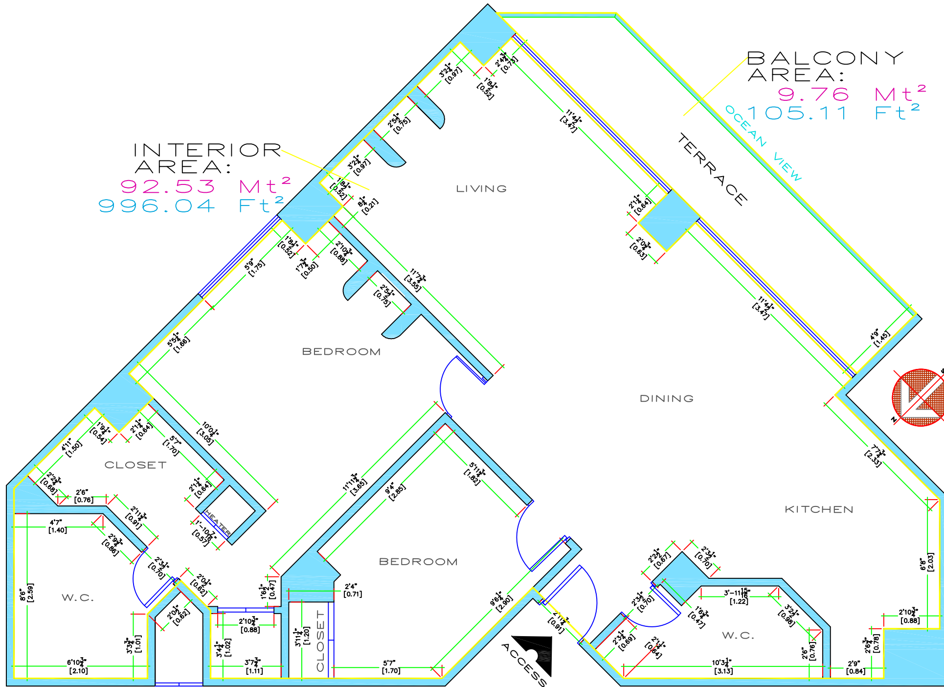
ARCHITECTURAL PLAN CM-1209 MEASURES
