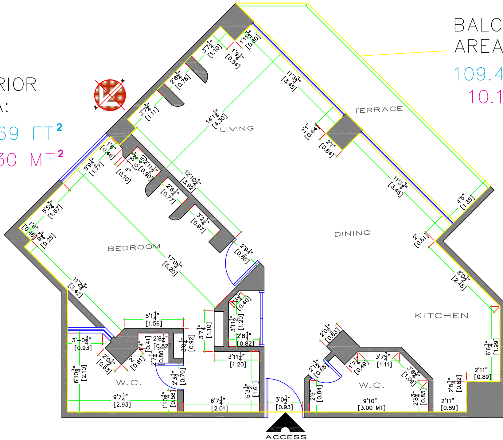
ARCHITECTURAL PLAN CM-109 MEASURE'S
