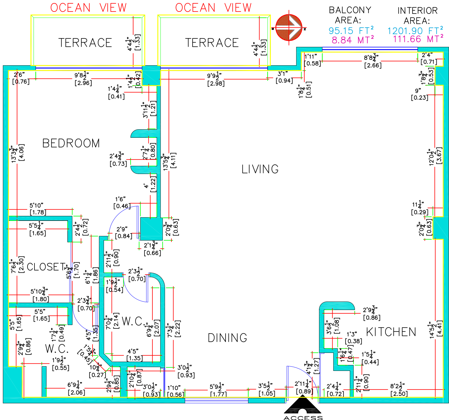
ARCHITECTURAL PLAN CM-103 MEASURE'S
